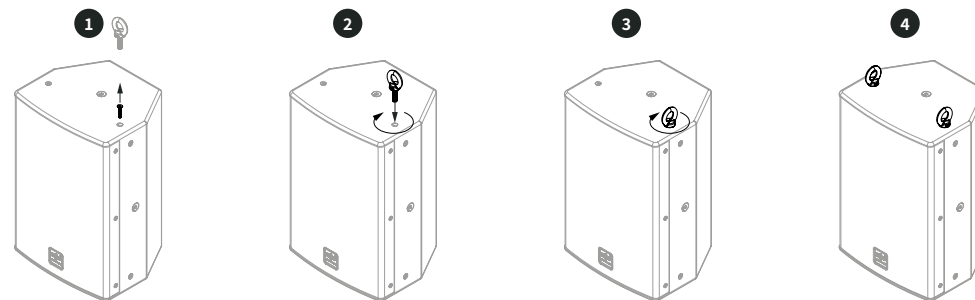
Figure 10. COX 8 MKII - Preparing for flown installation.
