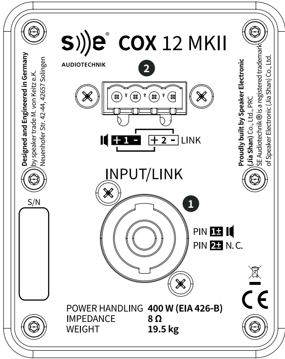
Figure 2. COX 12 MKII - Connection terminal.
