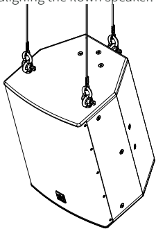
Figure 20. COX 8 MKII - Example of flown installation.
