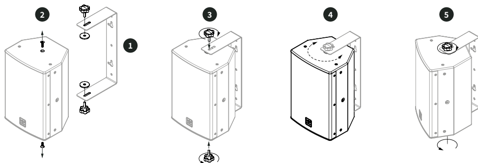
Figure 12. COX 8 MKII - COX 8 MKII - Installation with Wall Mount Bracket.
