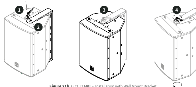
Figure 21b. COX 12 MKII - Installation with Wall Mount Bracket.
