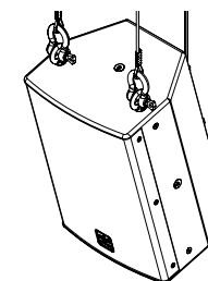
Figure 11. COX 8 MKII - Example of flown installation.
