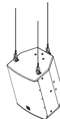
Figure 15. Hung from the ceiling using the M8 screw threads.
