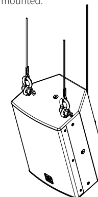
Figure 6. Hanged from the ceiling using the M5 and M8 screw threads.
